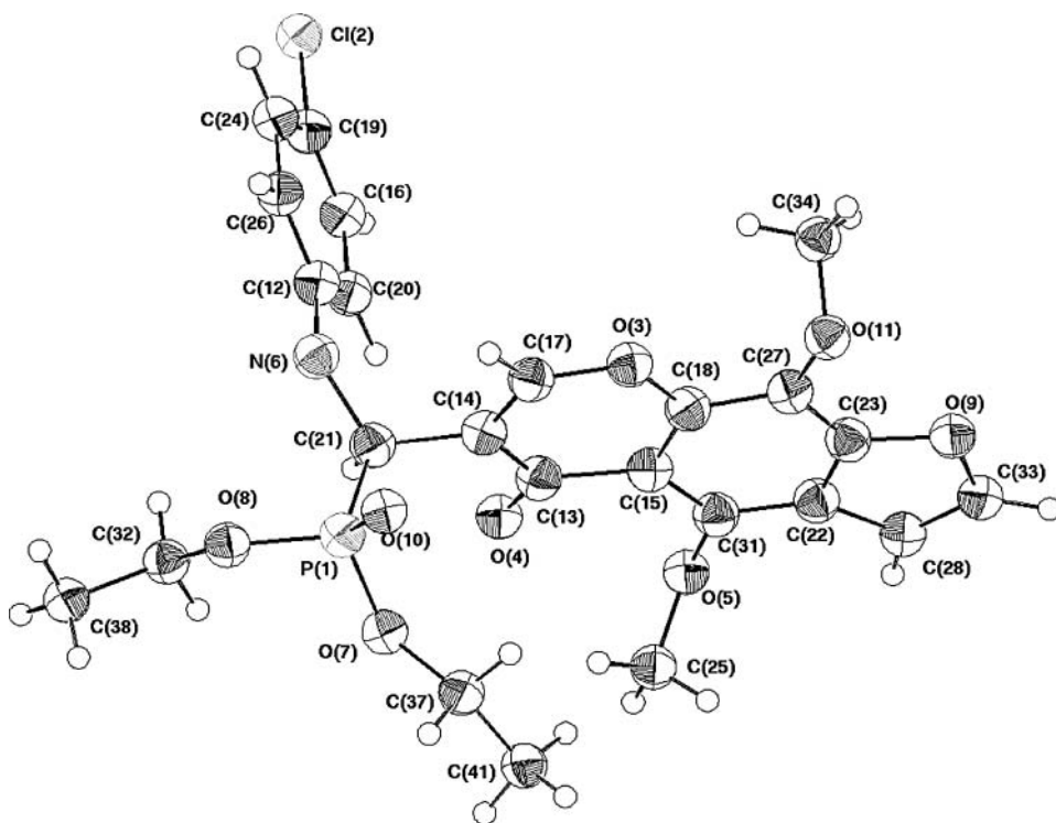
Figure 1 ORTEP projection of single X-ray diffraction of compound 5n .
